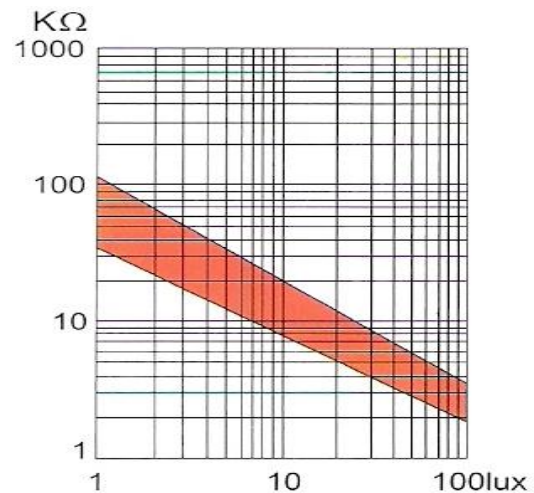
照度-电阻特性 ( Illuminance-resistance characteristics )
