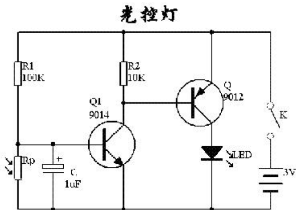
典型应用电路 ( Typical application circuit )
