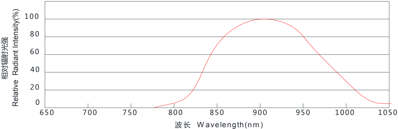
感光特性曲线 Photographic property Curve
