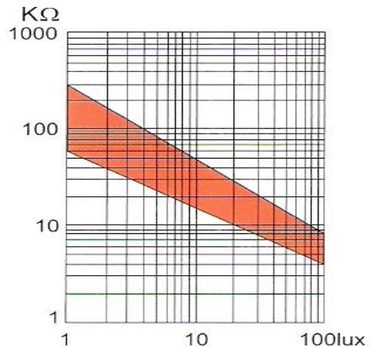
照度-电阻特性 ( Illuminance-resistance characteristics )
