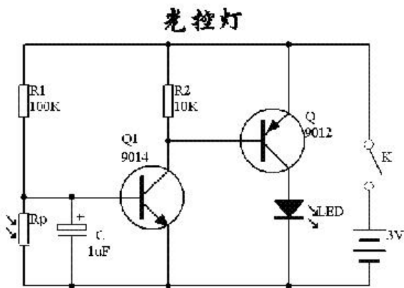
典型应用电路 ( Typical application circuit )
