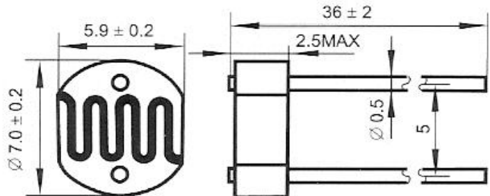
Overall dimension drawing (unit: mm)
