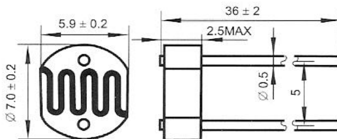
Overall dimension drawing (unit: mm)
