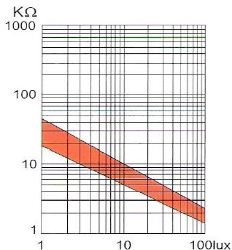
照度-电阻特性 ( Illuminance-resistance characteristics )
