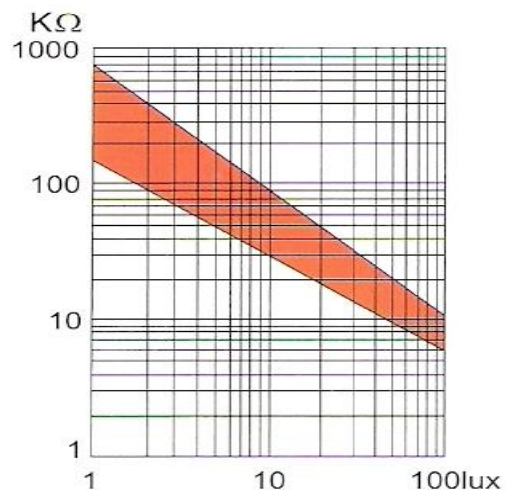
照度-电阻特性 ( Illuminance-resistance characteristics )
