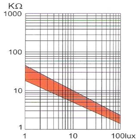
照度-电阻特性 ( Illuminance-resistance characteristics )
