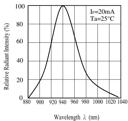
Fig.4 Relative Radiant Intensity vs.
