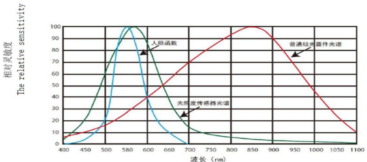
图 1-1 — Photoreceptor curve — HLPT550 — Visible light sensor curve
