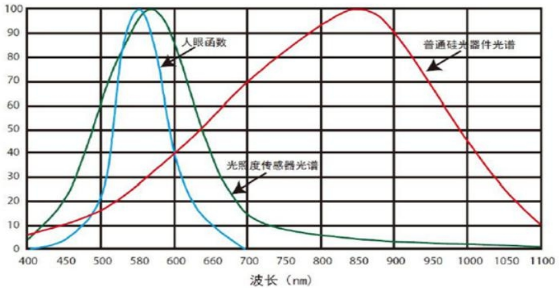
图 1-1 Photoreceptor curve HL5I560HP25 Visible light sensor curve
